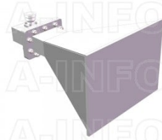
LB-284-15-C-7/16FSPO Standard Gain Horn Antenna 2.6-3.95GHz 15dB Gain 7/16(DIN) Female
